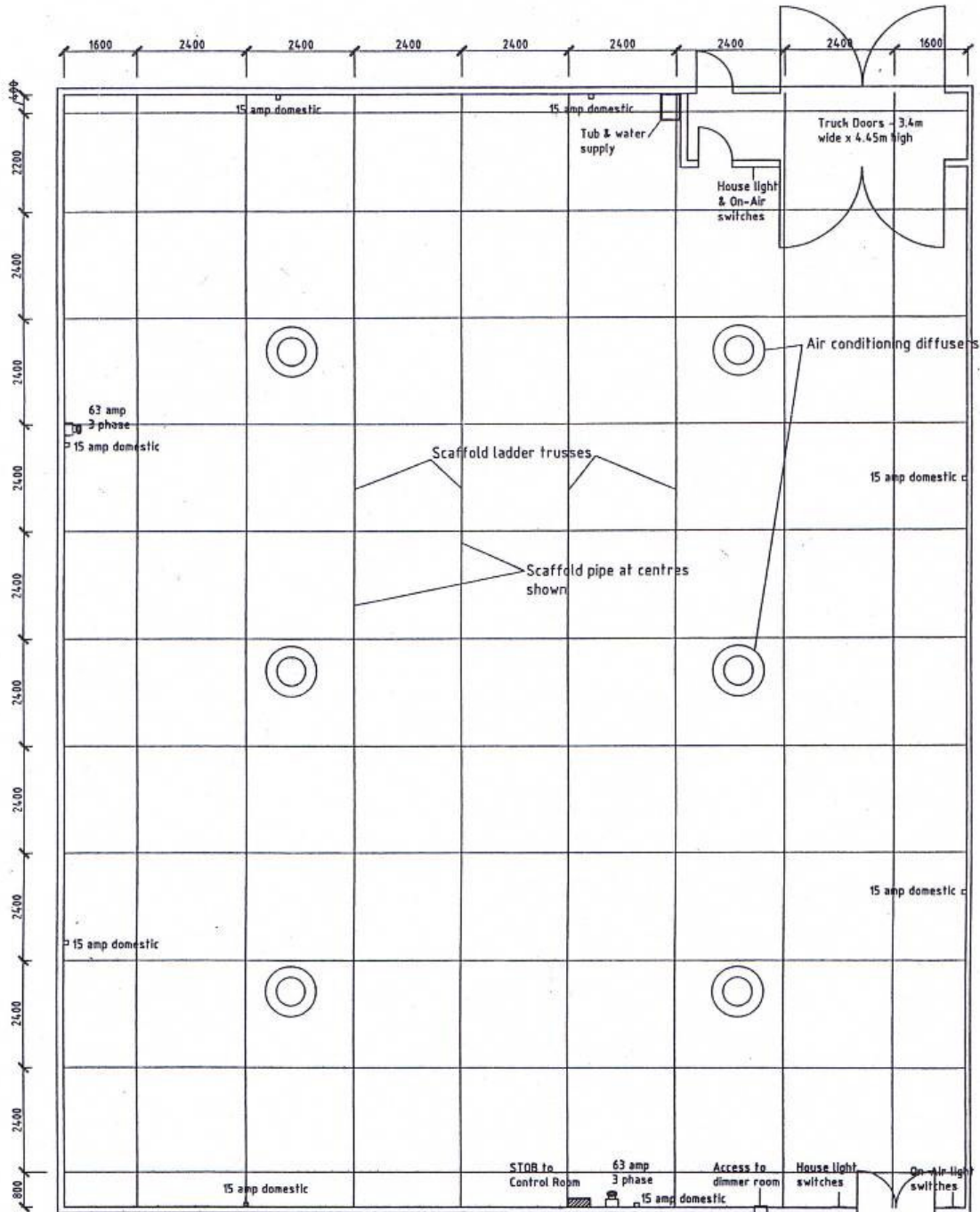
STUDIO TWO FLOOR PLAN Scale: 1:100
